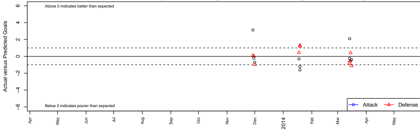
Players 98 Elite B97 Dots are actual minus expected GF (blue circles) and GA (red triangles). Blue line is smoothed change in attack strength. Red is smoothed change in defense strength.
